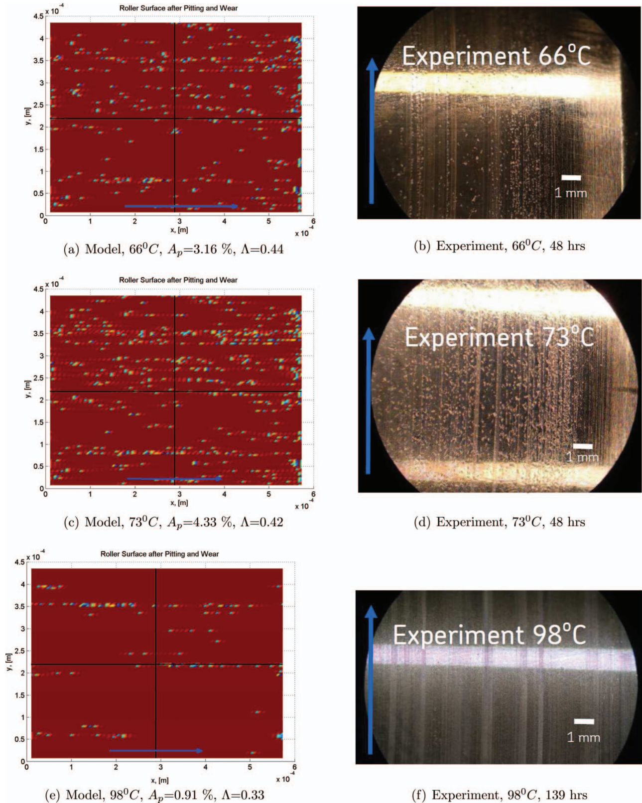
Fig. 14—Comparison of model results versus experiments in full bearing tests NU 211 ECP with artificially roughened surfaces: (a) calculation 66°C, (b) experiment 66°C, (c) calculation 73°C, (d) experiment 73°C, (e) calculation 98°C, (f) experiment 98°C. (color figure available online).
